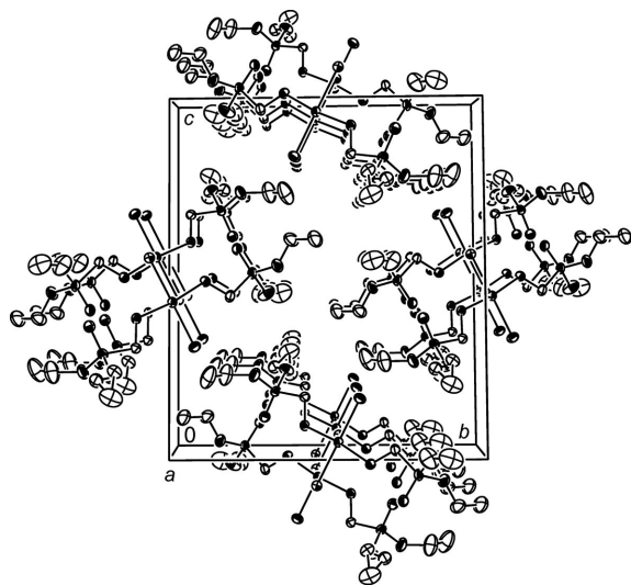
Figure 5. View of the crystal packing along the a axis of \text{trans-[PtCl}_2(\text{N-amp})_2] .
