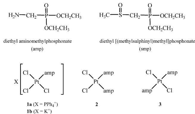
Scheme 1. Schematic view of the amp and smp ligands and of the complexes described in this paper.
