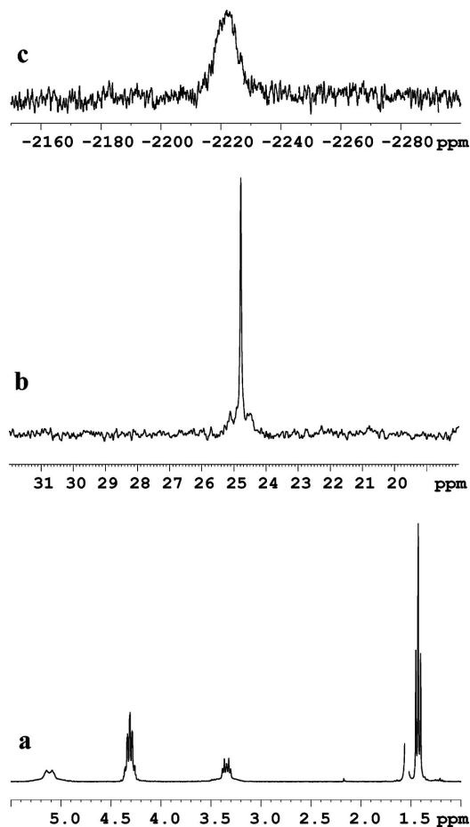
Figure 2. ^1H (a), ^{31}P (b), and ^{195}Pt NMR (c) spectra of compound 2 in CDCl_3 .
