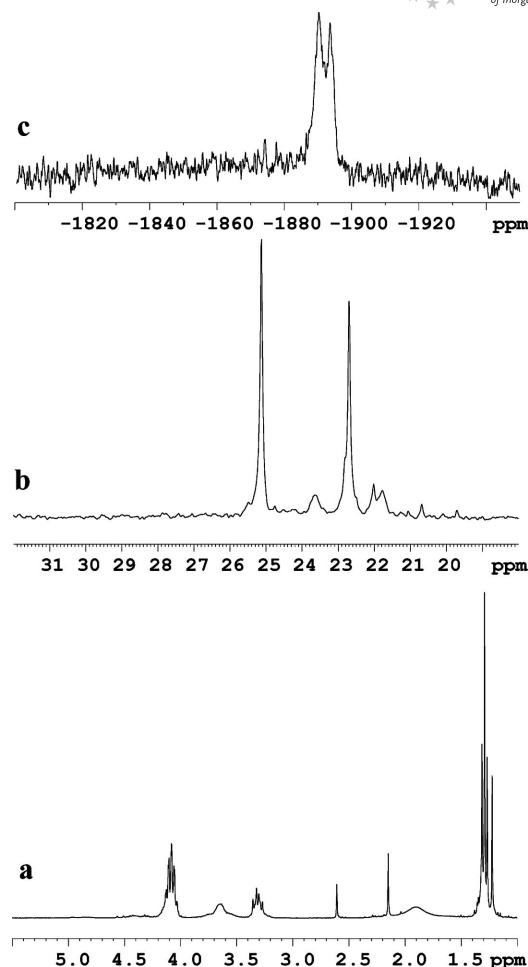
Figure 1. ^1\text{H} (a), ^{31}\text{P} (b), and ^{195}\text{Pt} NMR (c) spectra of compound 1a in \text{CDCl}_3 .
