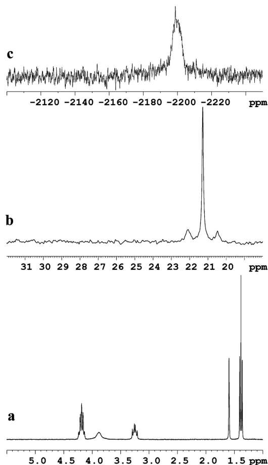
Figure 3. ^1\text{H} (a), ^{31}\text{P} (b), and ^{195}\text{Pt} NMR (c) spectra of compound 3 in \text{CDCl}_3 .
