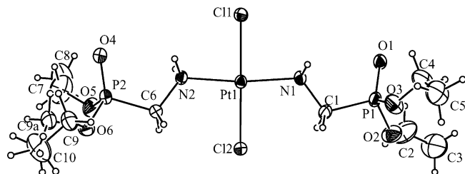
Figure 4. A view of the asymmetric unit of trans -[PtCl 2 ( N -amp) 2 ], showing the atomic numbering scheme. Displacement ellipsoids are drawn at the 30% probability level.
