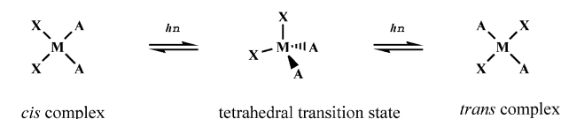
Scheme 2. Schematic view of the three possible \text{cis/trans} isomerization mechanisms.
